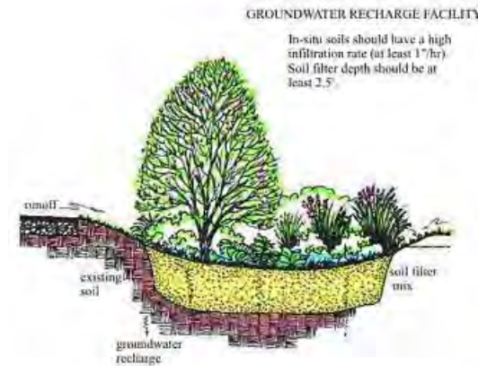
Figure 5-6: Bioretention Area
